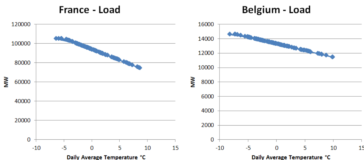
Figure 11 - Simulated temperature dependence of load for France (left) and Belgium (right)
