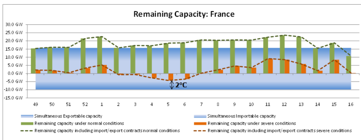
Figure 6 - Illustration of temperature sensitivity of margins (France)
