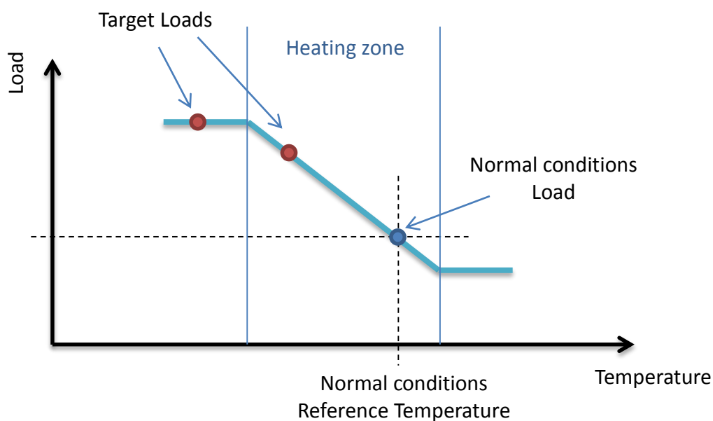
Figure 1 – Load temperature sensitivity
